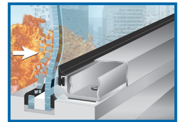
Madico FrameGard movement zone absorbs energy by allowing window film to stretch. Radius edge prevents cutting of film. Gripped surface clamps film in place.
